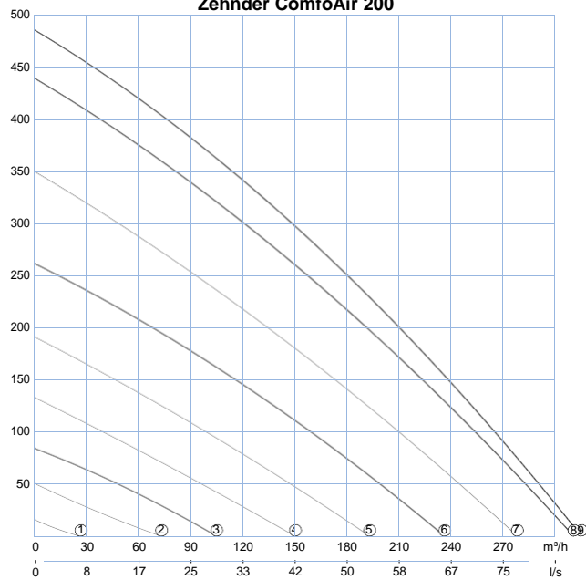
Zehnder ComfoAir 200
